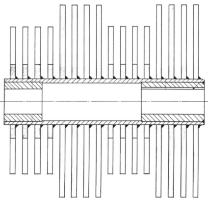
Lump Breaker blades and rotor configuration
