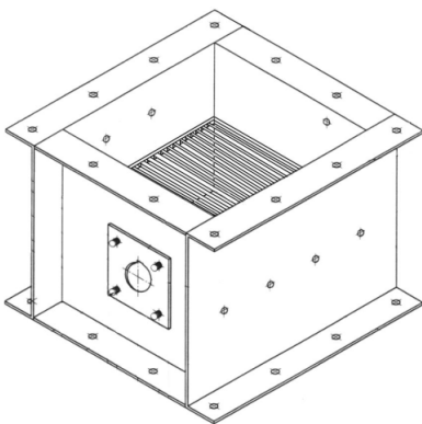
Lump Breaker body showing flanged ends and grill.
