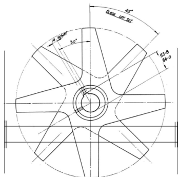
Lump Breaker blades configuration and impingement grill.
